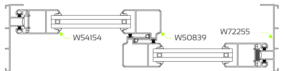
SECTION A-A Section not to scale
