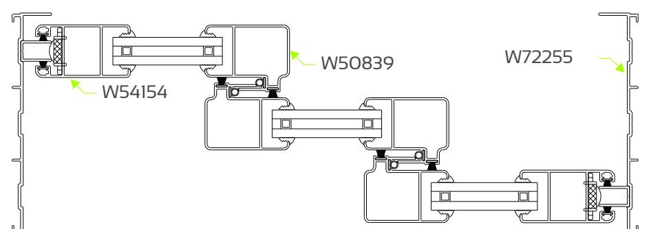
SECTION A-A Section not to scale
